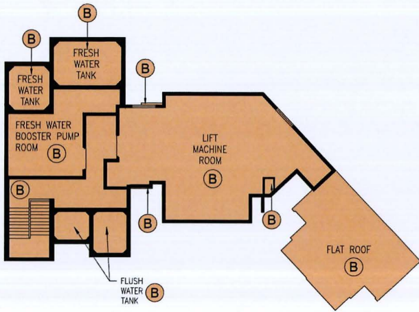
LIFT MACHINE ROOM PLAN
