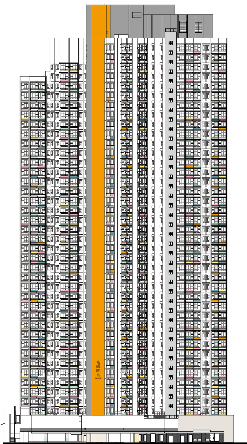
西南面立面圖 "3" South West Elevation Plan "3"
