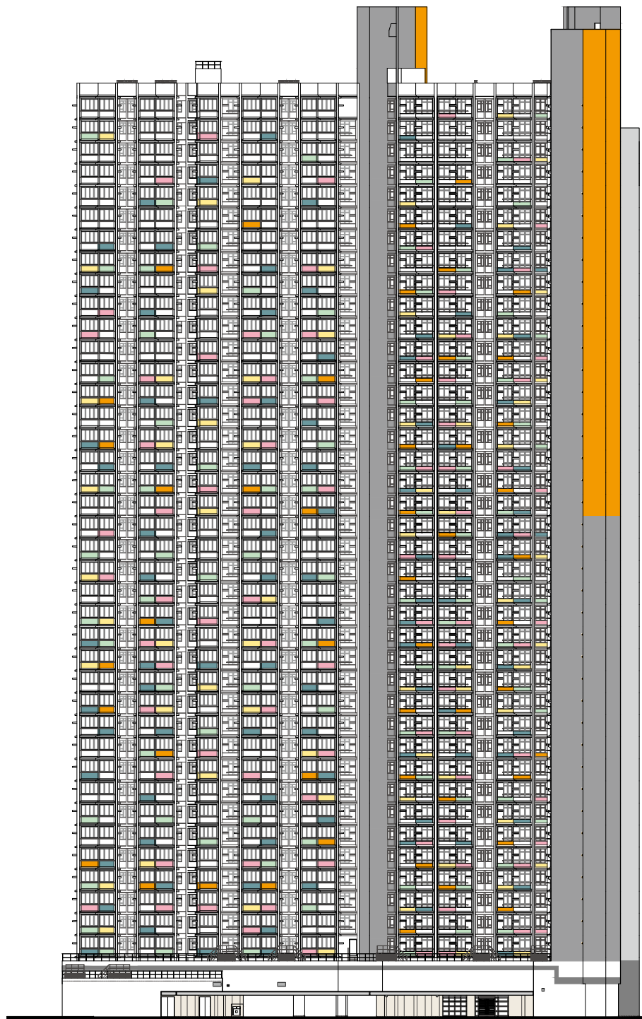
東面立面圖 "1" East Elevation Plan "1"
