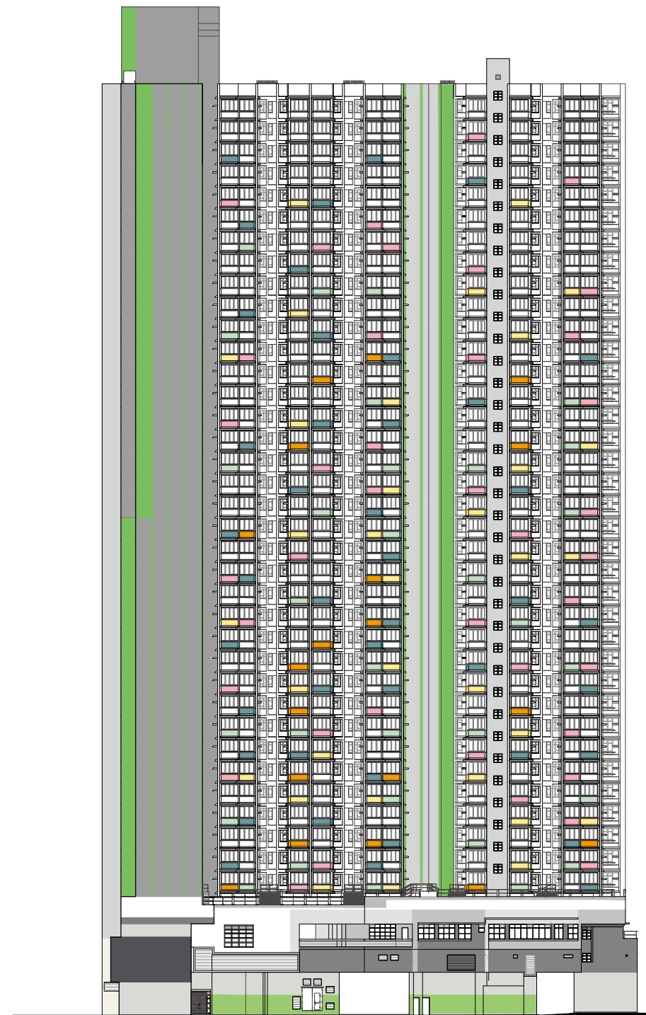
西北面立面圖 "2" North West Elevation Plan "2"
