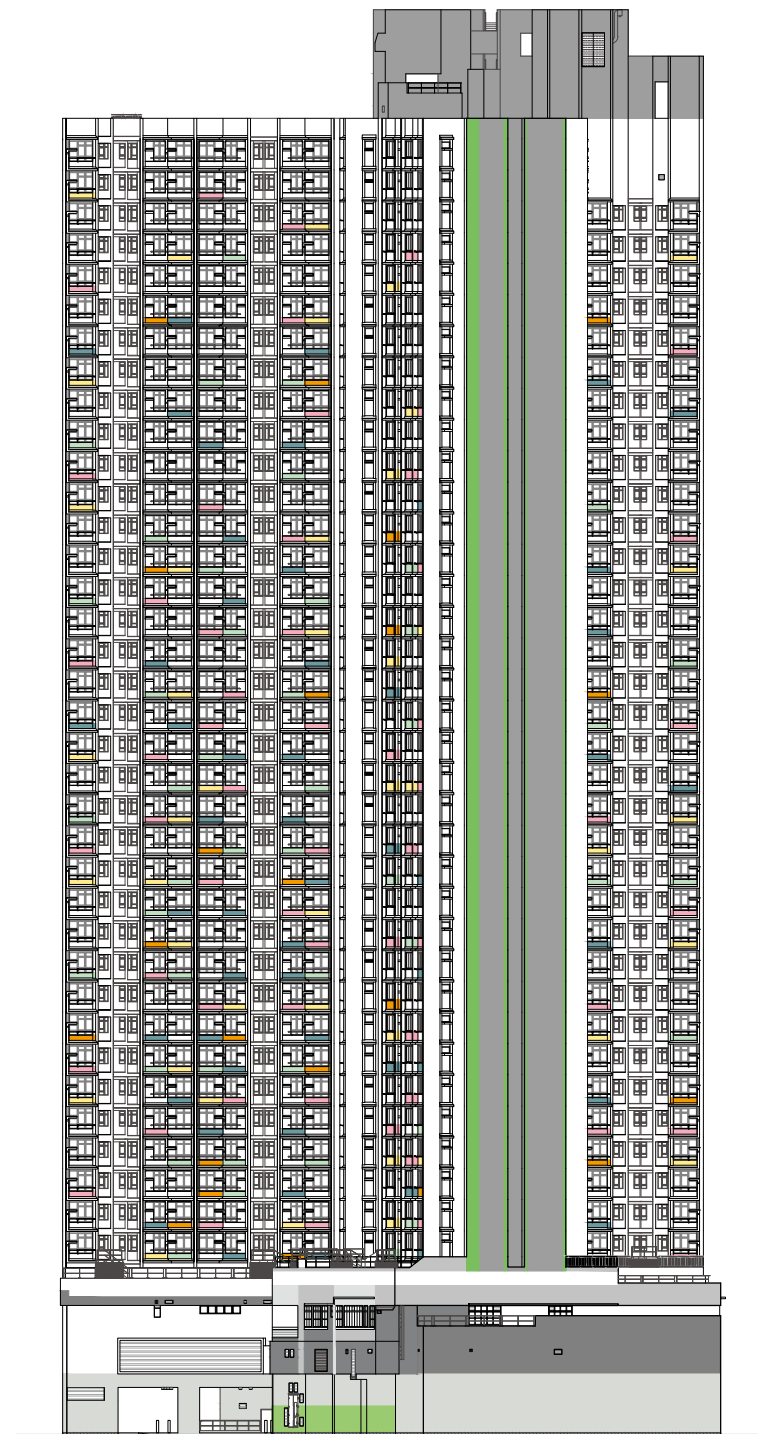
西南面立面圖 "1" South West Elevation Plan "1"
