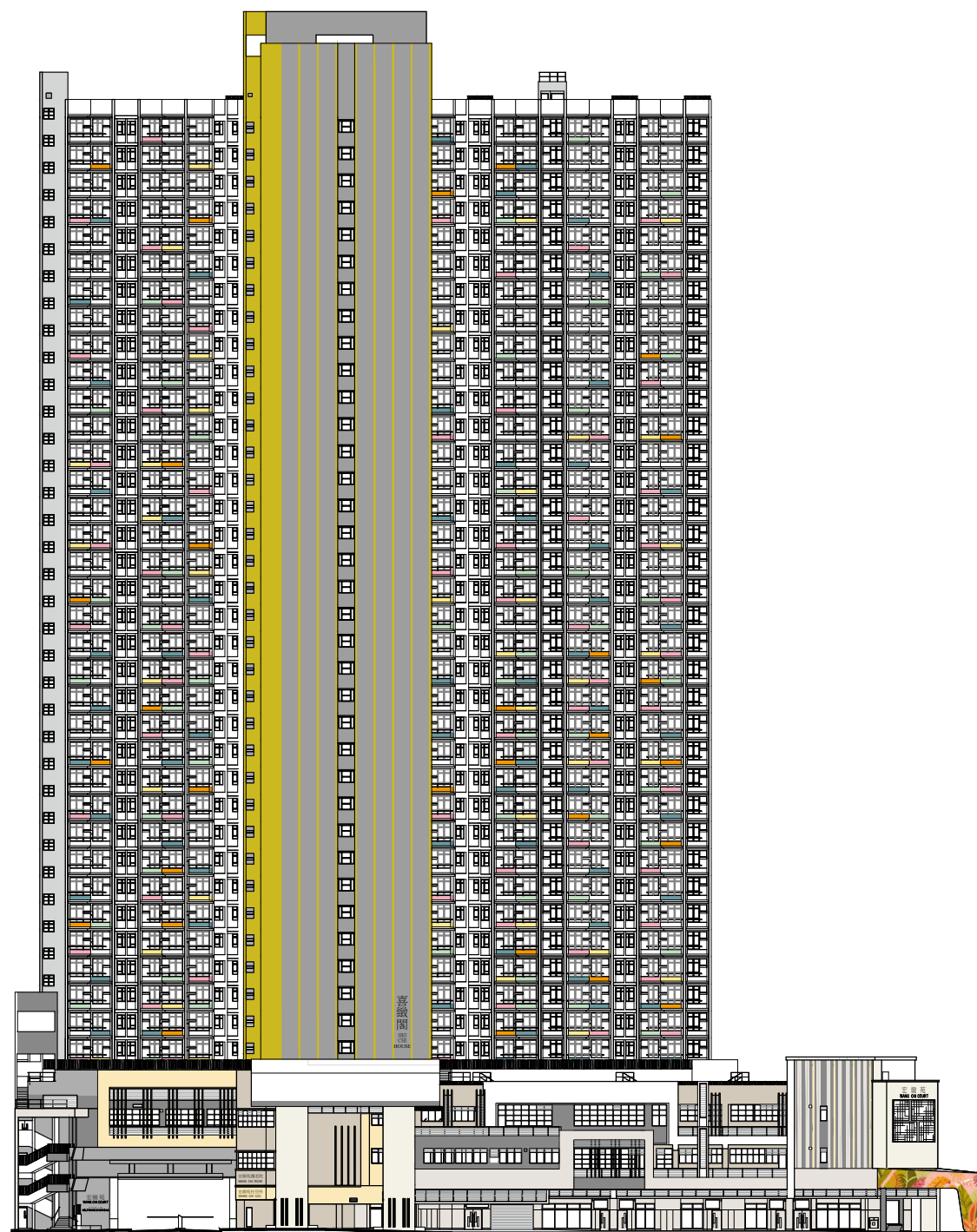
西南面立面圖 "1" South West Elevation Plan "1"
