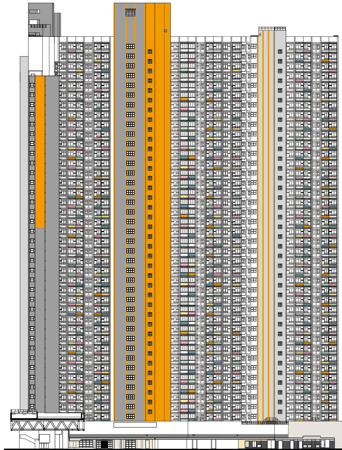
西面立面圖 "2" West Elevation Plan "2"
