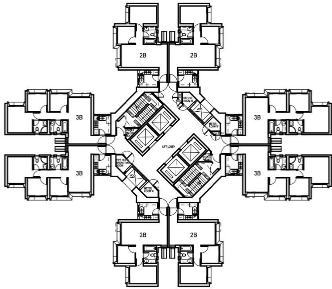
STANDARD BLOCK CONCORD 1 (OPTION 1) TYPICAL FLOOR PLAN
