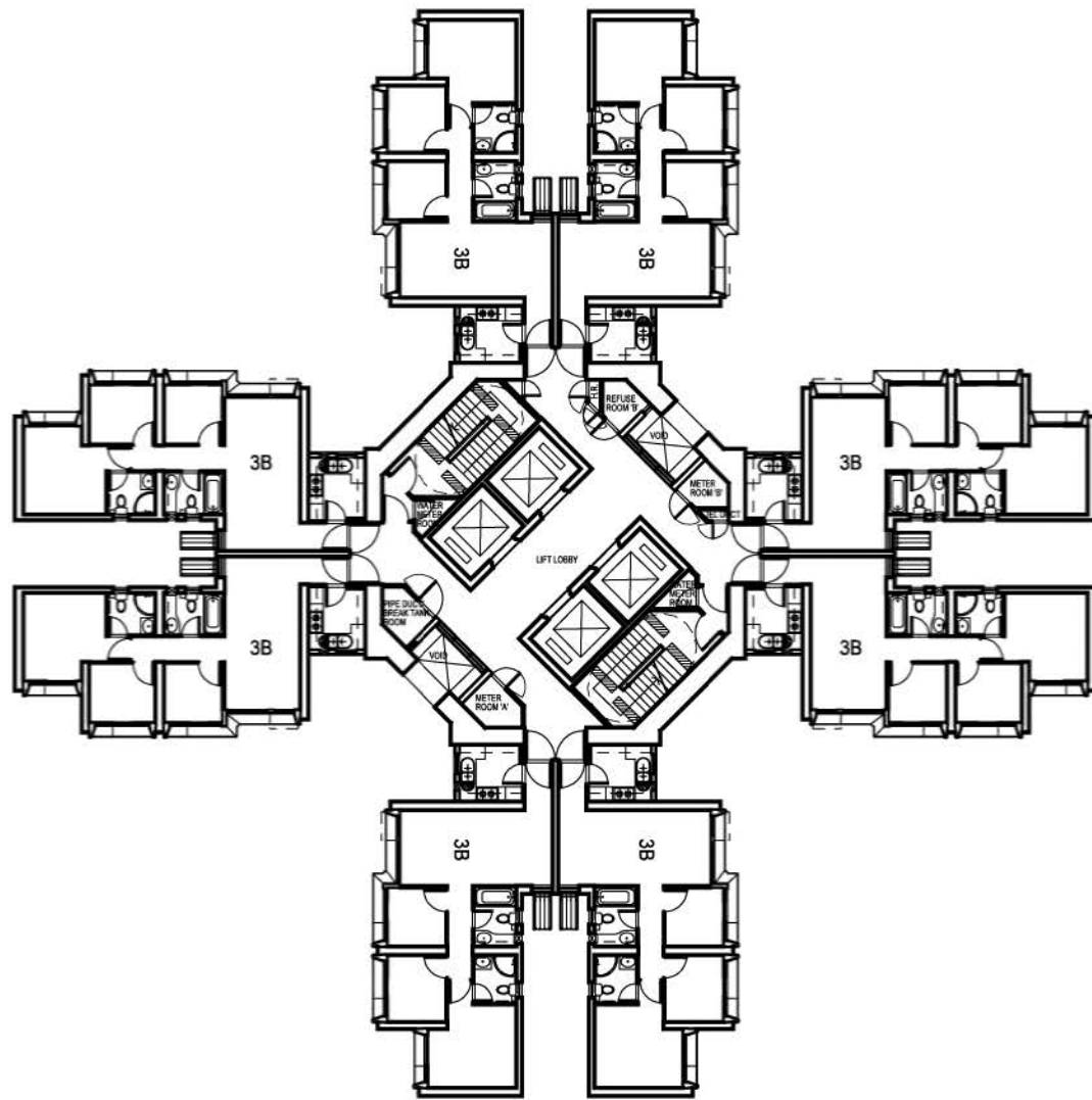
STANDARD BLOCK CONCORD 1 (OPTION 2) TYPICAL FLOOR PLAN
