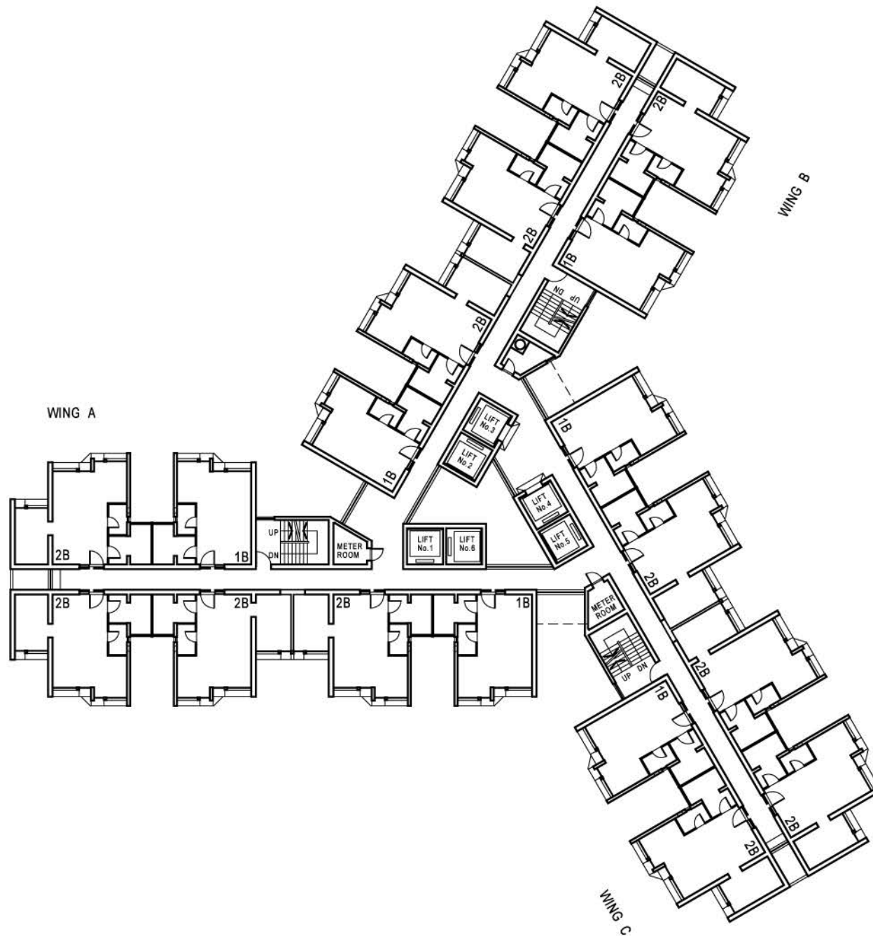
STANDARD BLOCK HARMONY 2 (OPTION 2 & 5) TYPICAL FLOOR PLAN
