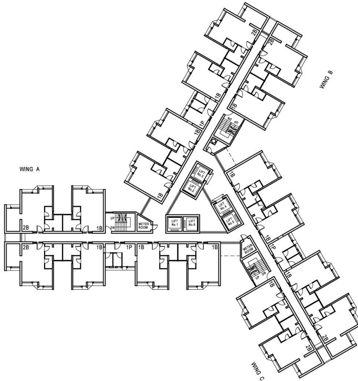
STANDARD BLOCK HARMONY 2 (OPTION 3) TYPICAL FLOOR PLAN
