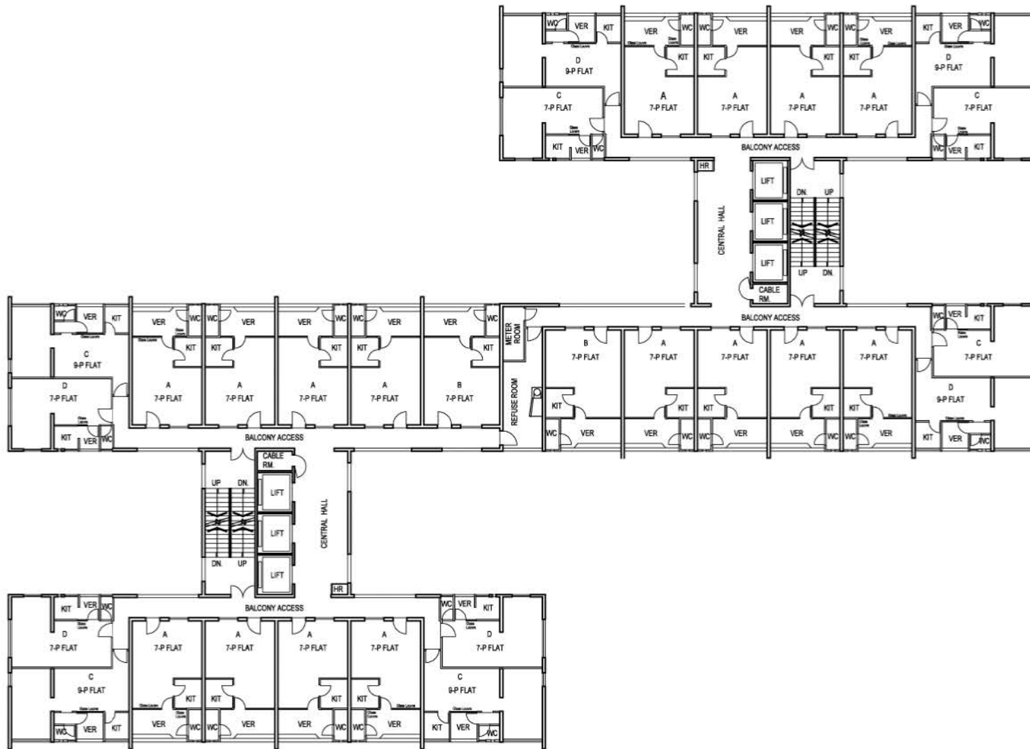
STANDARD BLOCK TWIN - H TYPICAL FLOOR PLAN
