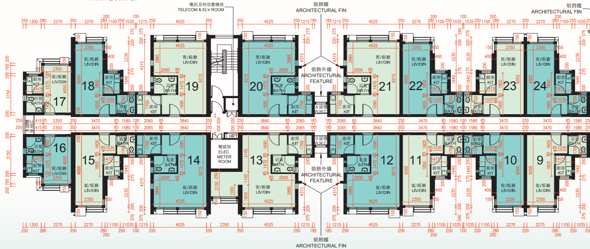
3樓部分平面圖 PART PLAN AT 3/F
