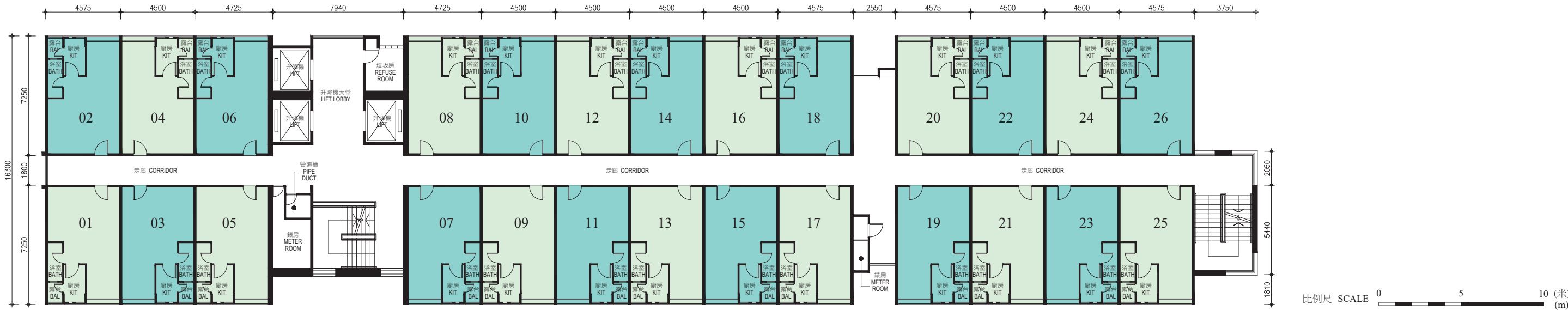
18及19樓部份平面圖 PART PLAN OF 18/F AND 19/F
